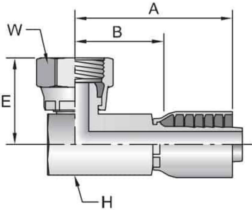
1B4GM BSPP Female - 90° Block Type Elbow Swivel (60° Cone)
