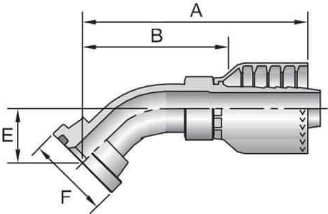
117MH SAE Code 61 Flange Head - 45° Elbow
