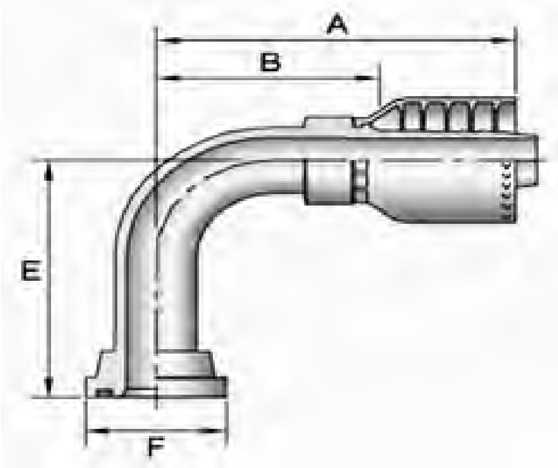
189GM SAE Code 61 Flange Head 90° Long Drop Elbow
