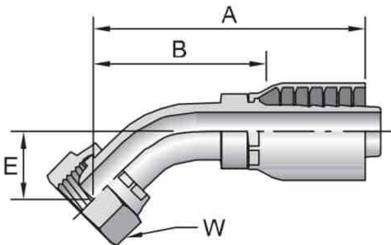
1C0MH Metric H Female - 45° Elbow Swivel (24° Cone with O-Ring)
