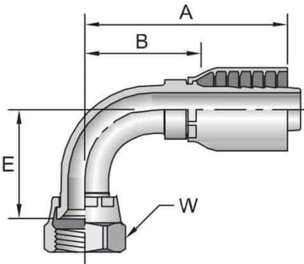
139MH Female JIC 37° - 90° Elbow Swivel
