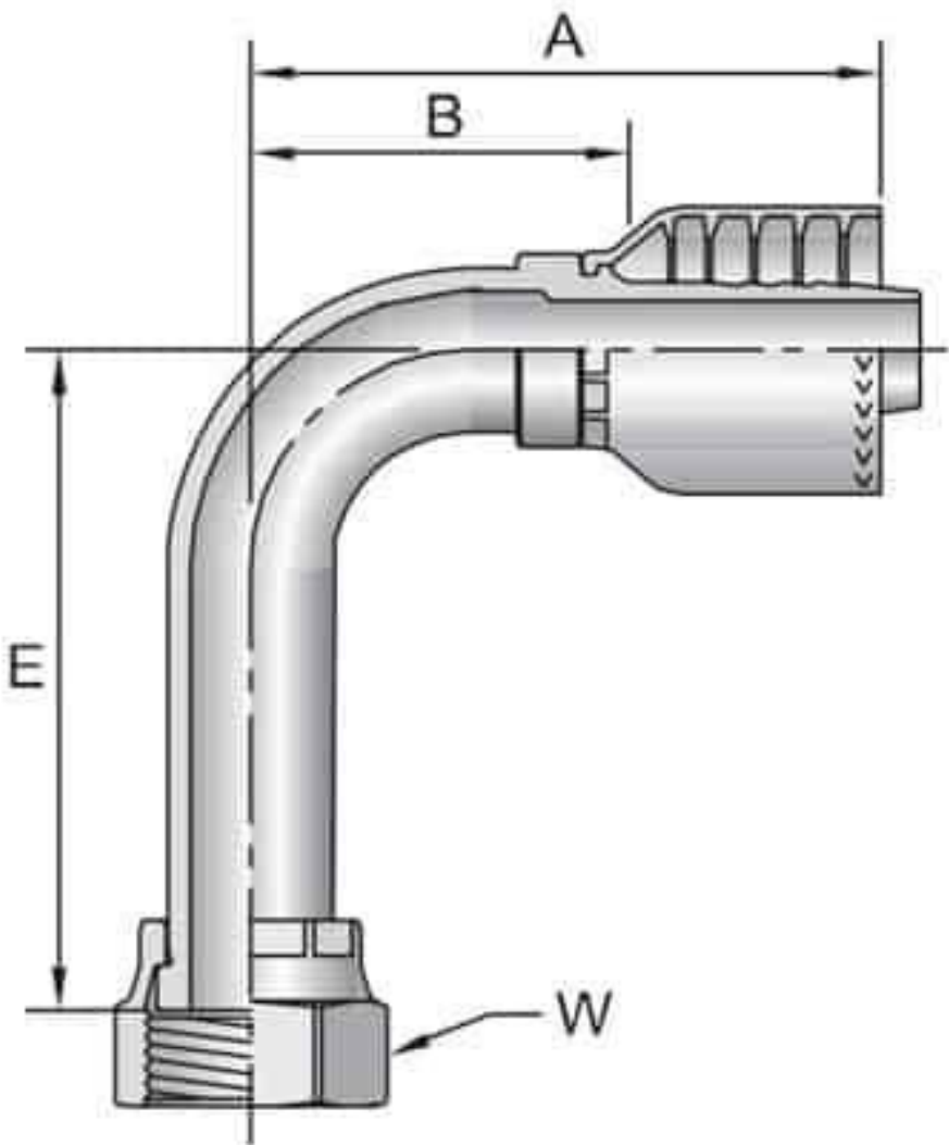
1J1GM Female ORFS Flat Face - 90° Long Drop Elbow Swivel
