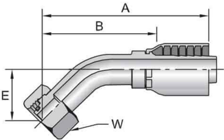
1C0GM Metric H Female - 45° Swivel (24° Cone with O-Ring)
