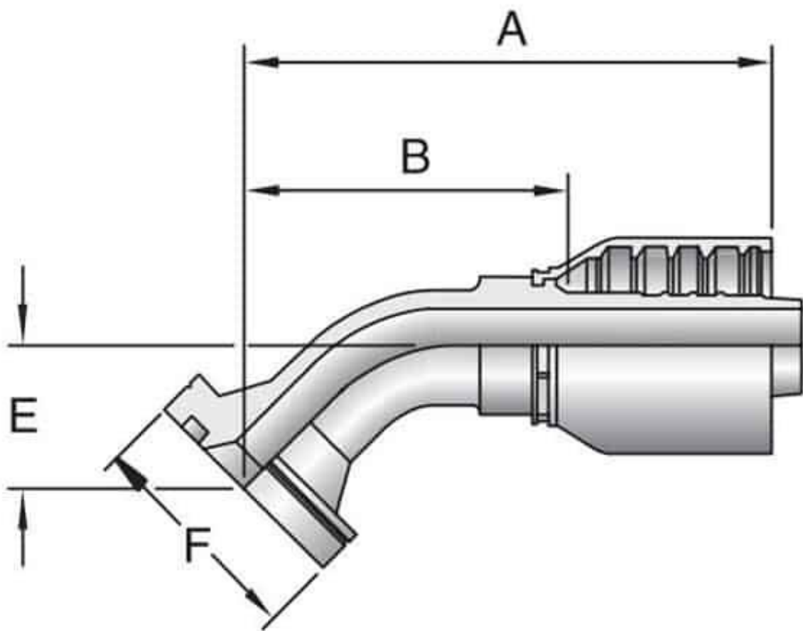
16FGM SAE Code 62 Flange Head - 45° Elbow
