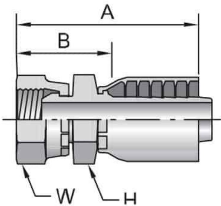
102GM Female NPT Pipe - Swivel
