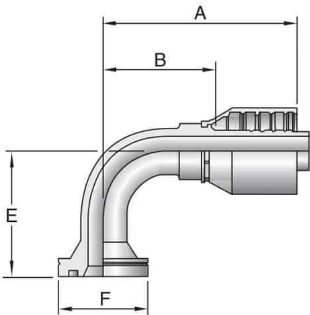
16NGM SAE Code 62 Flange Head - 90° Elbow
