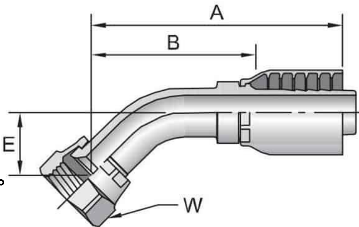
137MH Female JIC 37° - 45° Elbow Swivel
